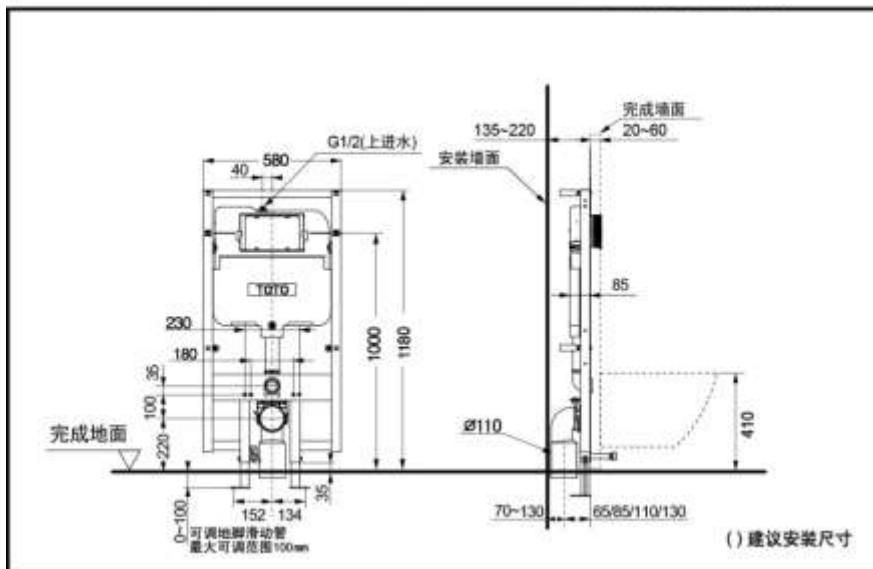
WH173BT-562EB WH173BT-572EB Concealed Flush Tank
