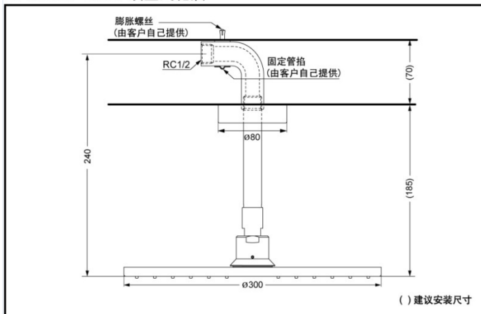
DBX113-1CA 顶置式花洒
