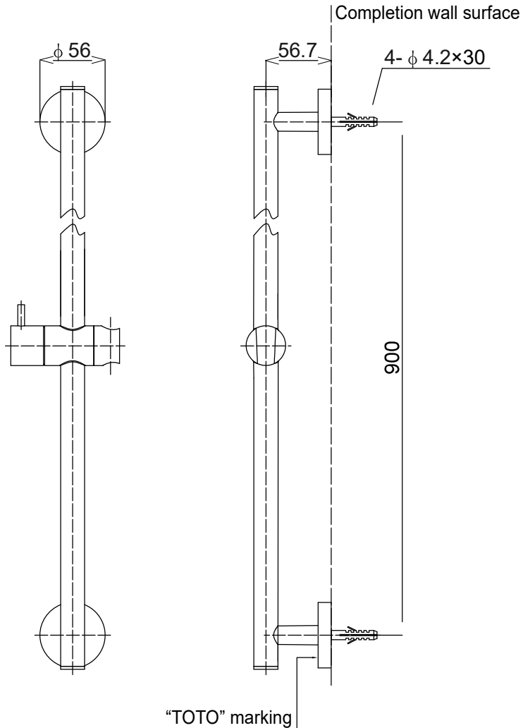
TBW01015* "L Shower" Sliding Rail 900 (Standard Type)
